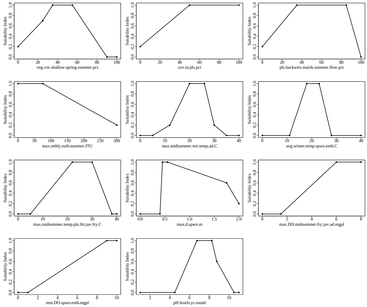
Figure 1. Suitability index graphs for variables included in the commoncarpRivNoSal model in ecorest.
